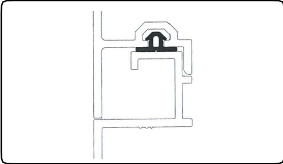
005 GASKET DETAIL OF PROFILE (NO FUGA*)
